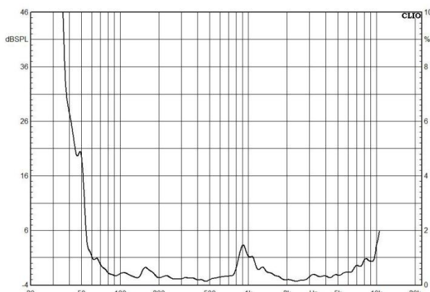
Distortion (THD < 2% 1W, 1m, 100Hz-10kHz)
